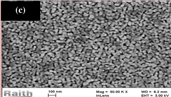
Top-view SEM images of TiO 2 thin films
