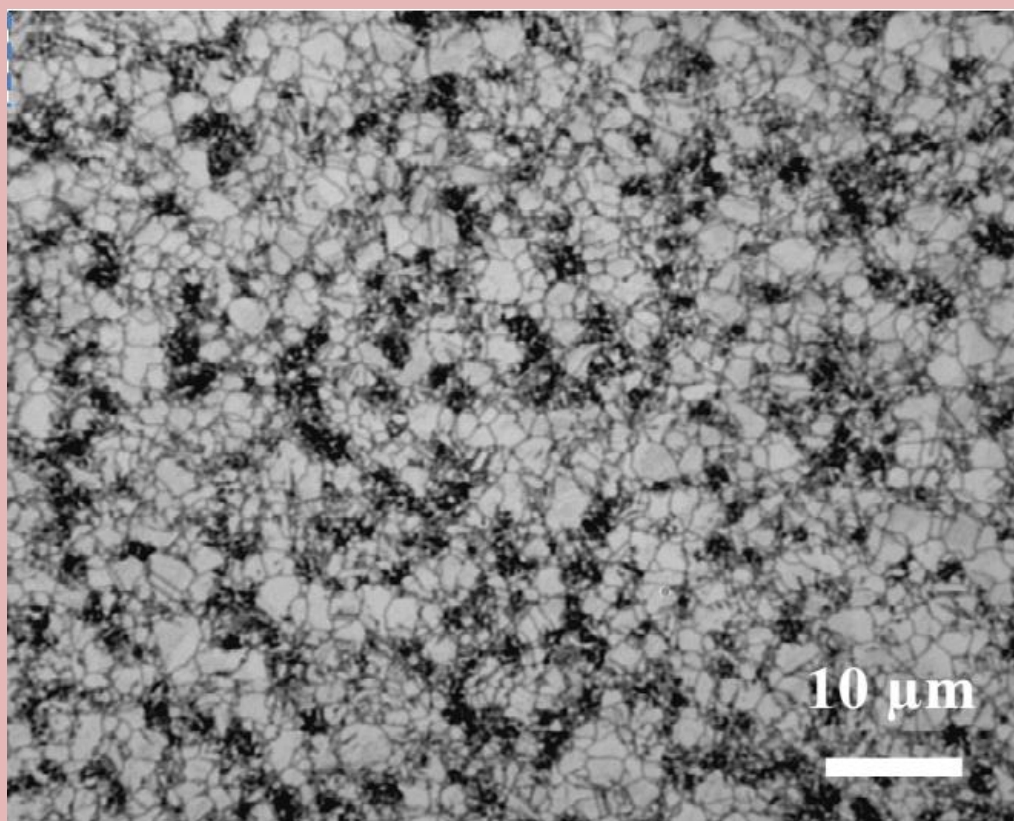
Surface image of a polysilicon layer deposited by RTCVD
