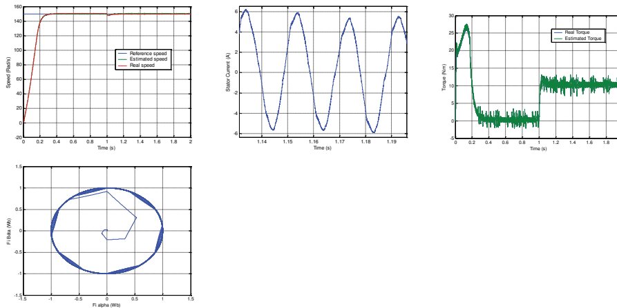
Fig.5. without speed sensor DTC by EKF applied to the linear model
