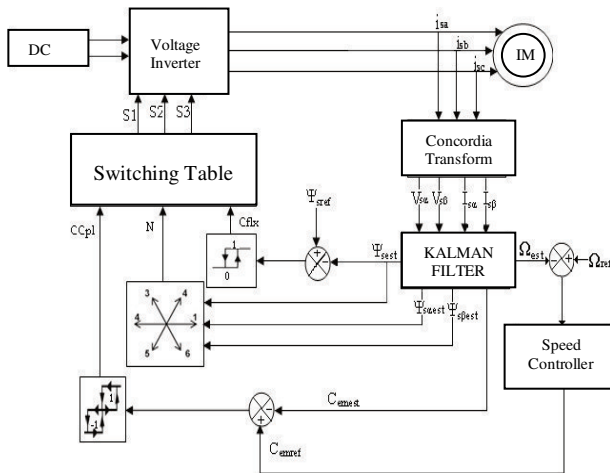
Fig.4. General structure of the direct torque control without mechanical sensor by the use of the extended KALMAN filter
