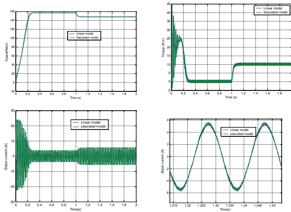
Fig.1. Start up following by a load application of an induction motor: linear model (blue curve), saturated model (green curve)
