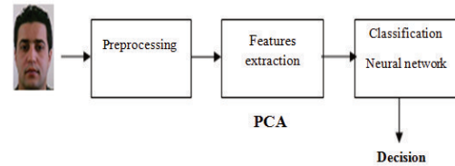
Fig 9. Neural-PCA system
