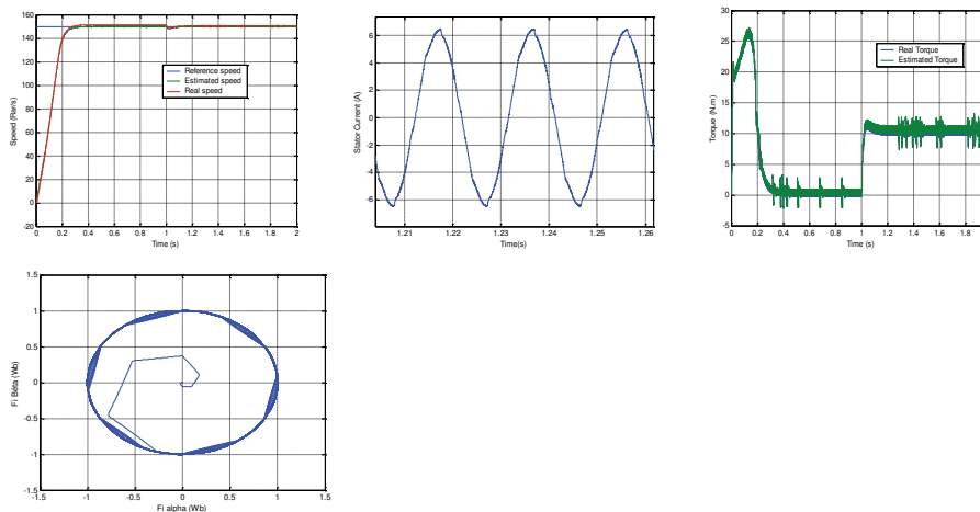
Fig.6. without speed sensor DTC by EKF applied to the saturated model
