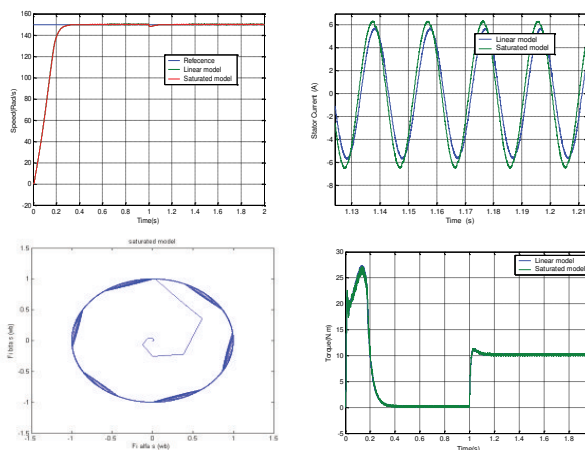
Fig.3. DTC of the induction motor: nominal reference speed and nominal load application
