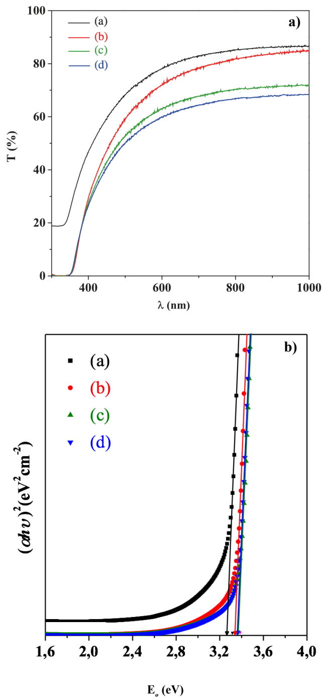
Fig. 1. UV-Vis and Tauc plots of undoped \text{TiO}_2 on ITO : (a) 3 layers, (b), 5 layers (c), 10 layers and (d) 15 layers.
