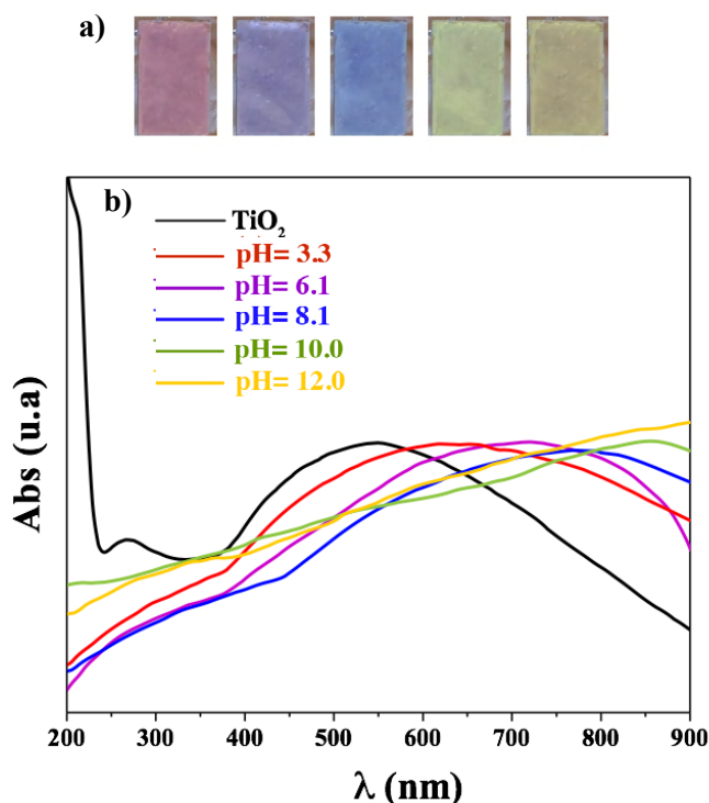
Fig. 4. a) TiO 2 photoanodes sensitized with anthocyanin at different pH. b) Uv-visible spectrum of TiO 2 and TiO 2 layers sensitized with pigment at different pH.
