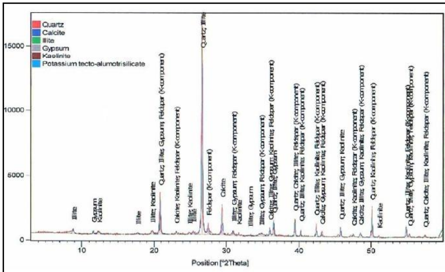
Figure 1 : Mineralogical analysis of bricks in earth of the walls of the ksour Tinerkouk – Adrar
