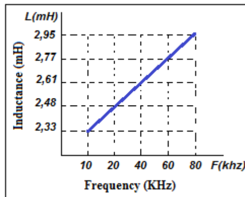
Fig. 10. Frequency sweep and the influence of inductance.
