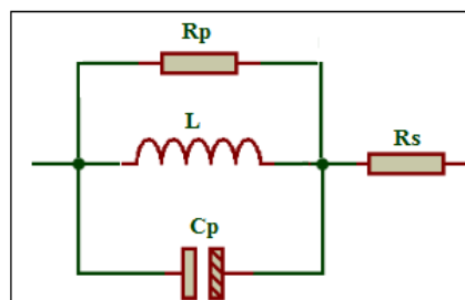
Fig. 7. Equivalent model of impedance Z.
