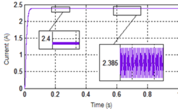
Fig. 13. The output current I_s of boost converter.
