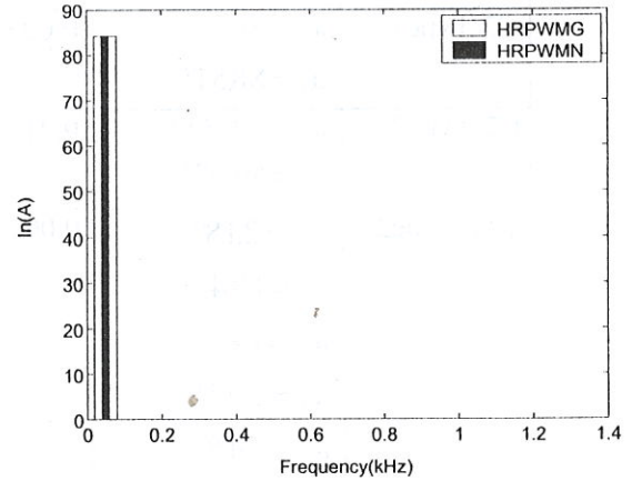
Figure 13. Spectre of input current of ac/dc converter (HRPWMN, HRPWMG, control C11 type 2).
