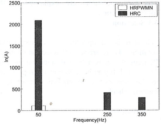
Figure 7. Spectre of input current of ac/dc converter (Conventional, HRPWMN, control C2, type 1).
