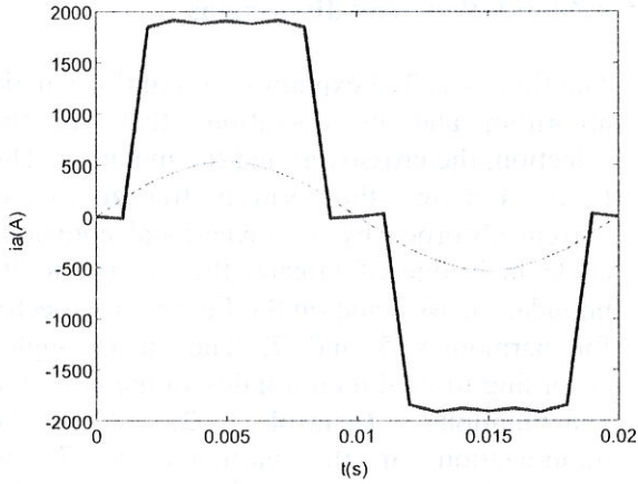
Figure 4. Input current and voltage of conventional ac/dc converter
