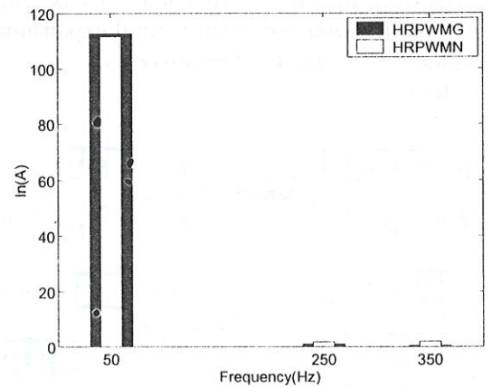
Figure 8. Spectre of input current of ac/dc converter (HRPWMN, HRPWMG, control C2, type 1).
