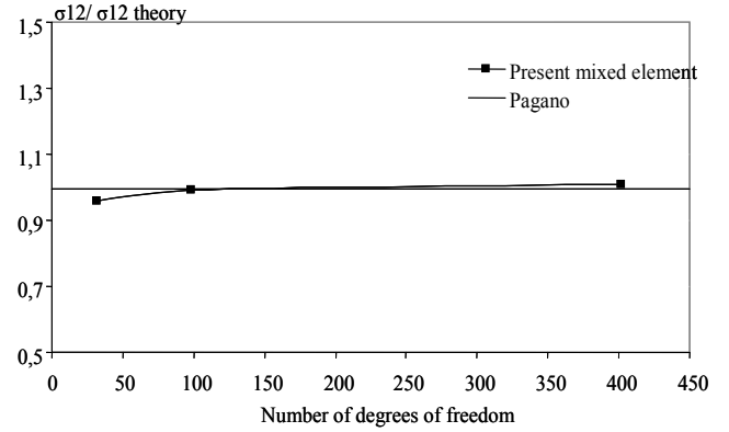
Figure 6 : Convergence of transverse shear at x=L/4 ( y = -h/2 )
