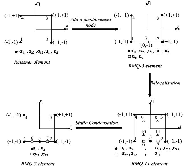
Figure 1 : Stages of construction of RMQ-7 element
