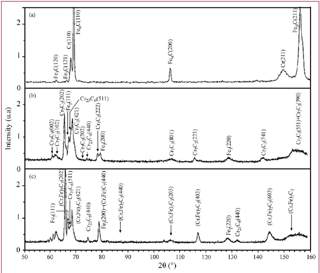
Figure 1: X-ray diffraction spectra of the samples [Cr(3 \mu m)/100C6 steel] before (a) and after annealing during 30 min at 900°C (b) and 1000°C (c).
