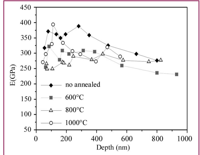
Figure 3: Evolution of Young modulus with analysed depth.
