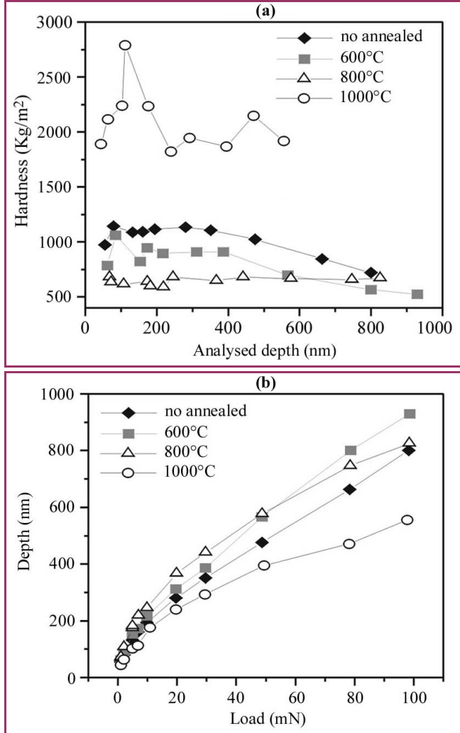
Figure 2: Nanoindentation measurements.
