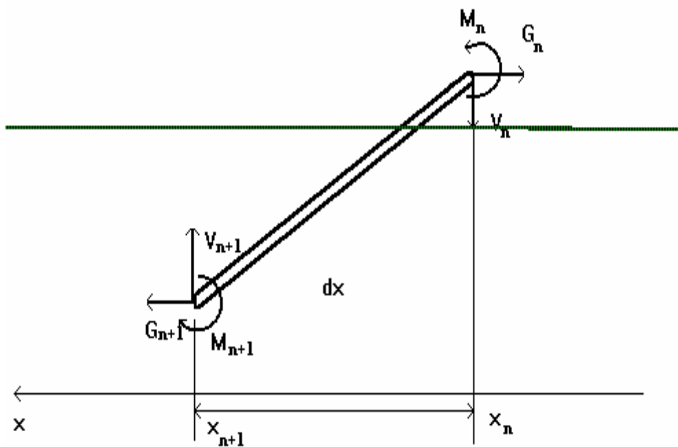
Fig. 2: Blade element equilibrium
