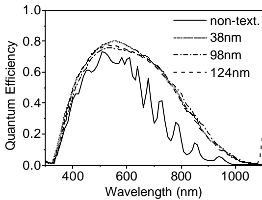
Fig. 6: Quantum efficiency for pin solar cells deposited on differently rough ZnO substrates measured at -1 V.
