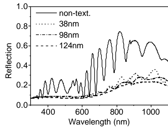
Fig. 7: Reflection of pin solar cells deposited on differently rough ZnO substrates.
