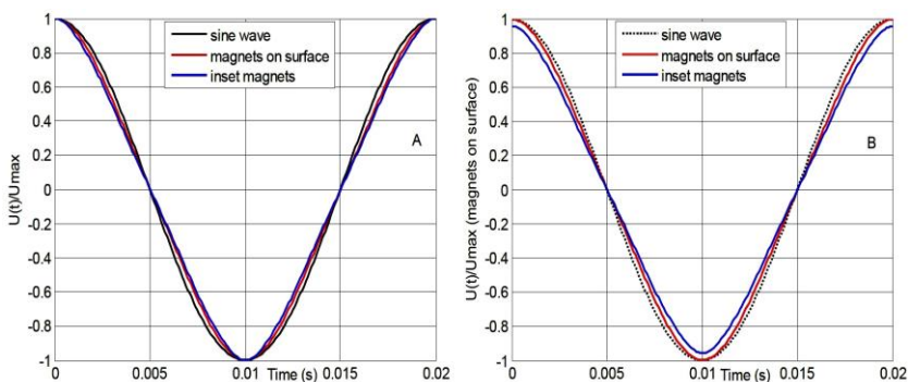
Fig. 4: Effect of magnets location on the generated voltage (A): Distortion, (B): Magnitude
