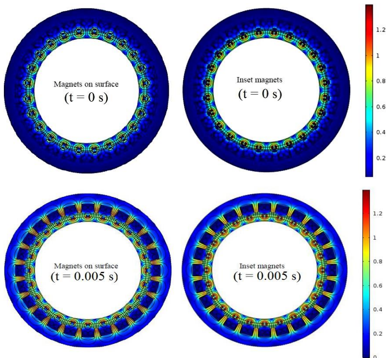
Fig. 3: Magnetic flux density distribution and magnetic potential vector contours calculated in permanent magnet generators; with magnets on rotor surface and inset magnets type
