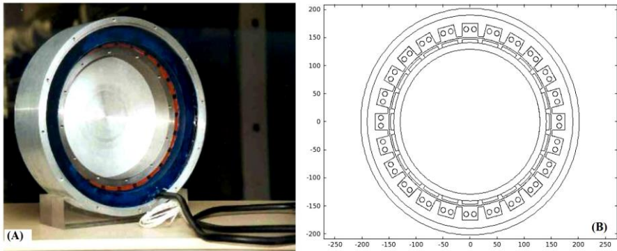
Fig. 1: Permanent magnet generator, (A): Photo [8], (B): Diagram of the generator cross section, where the dimensions are taken from reference [8]
