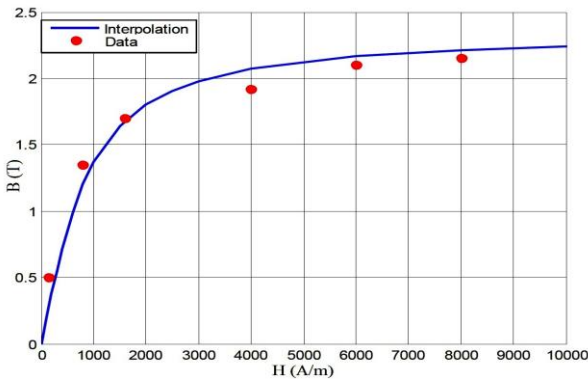
Fig. 2: Magnetization characteristic curve of Iron-Cobalt Alloy ( B_s = 1.36T , k = 0.0012886m/A )
