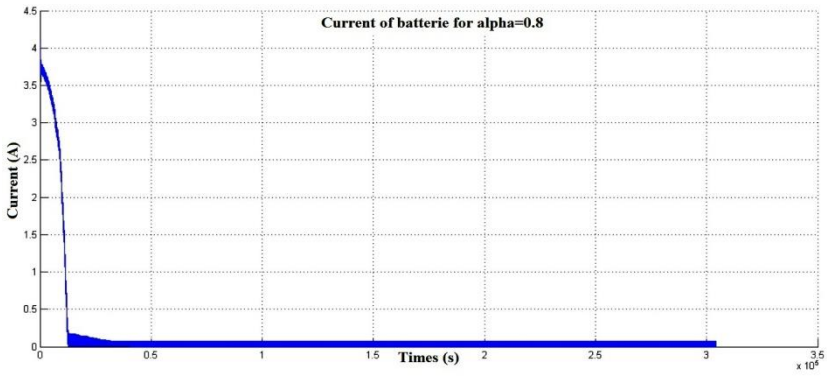
Fig. 6: Simulations show the courant of the batterie for duty cycle \alpha = 0.8
