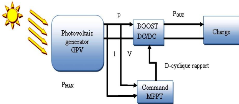
Fig. 3: Representation of the circuit electronic
