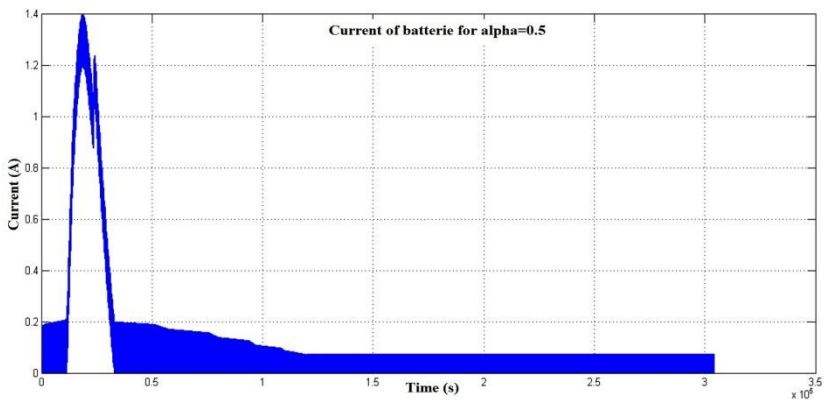
Fig. 4: Simulations show the courant of the battery for duty cycle alpha = 0.5
