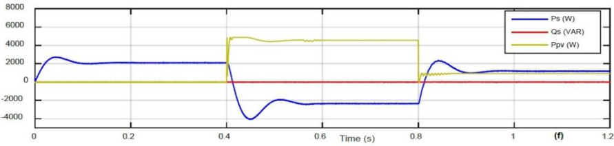
Fig. 10: Simulation results after compensation (to continue) (f) Active and reactive powers of source
