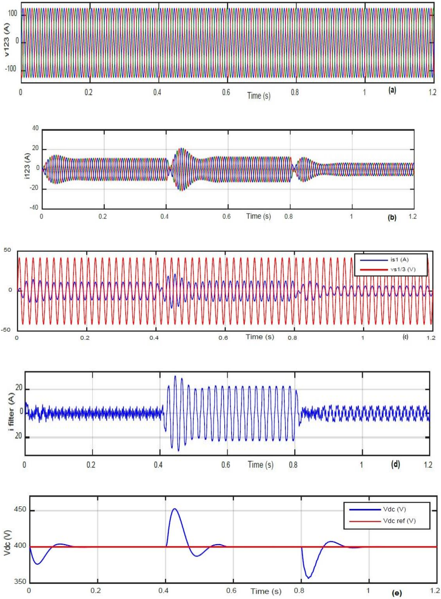
Fig. 10: Simulation results after compensation
