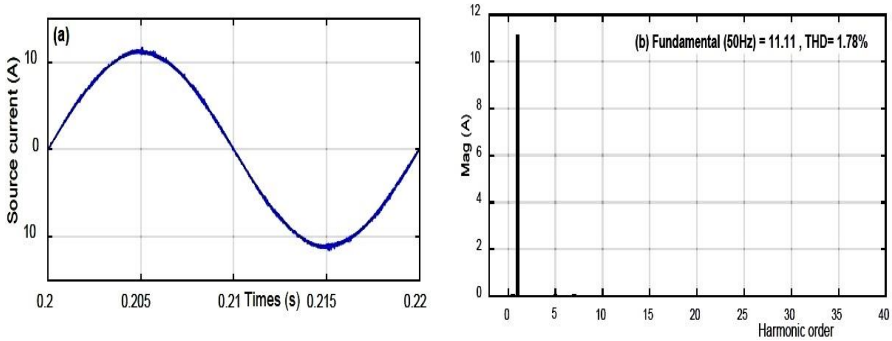
Fig. 11: (a) Supply current after harmonics compensation (b) current harmonic spectrum
