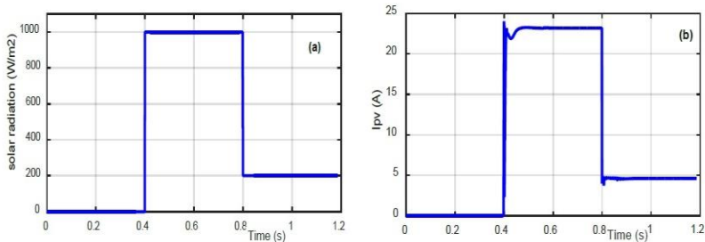
Fig. 9: (a) Solar radiation, (b) Current PV array
