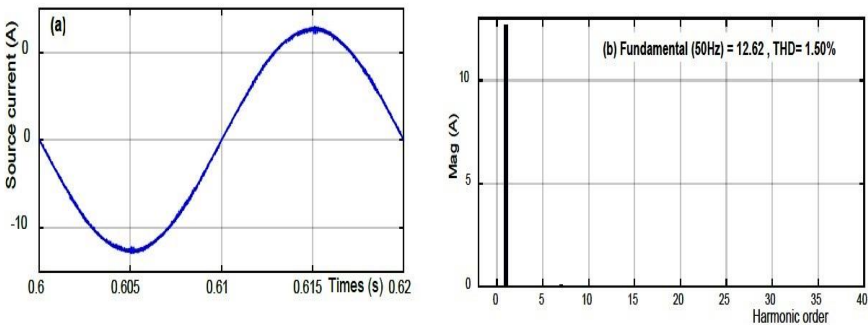
Fig. 12: (a) Supply current after harmonics compensation (b) current harmonic spectrum
