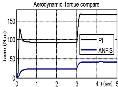
Fig. 8: Vehicle aerodynamic torque compare
