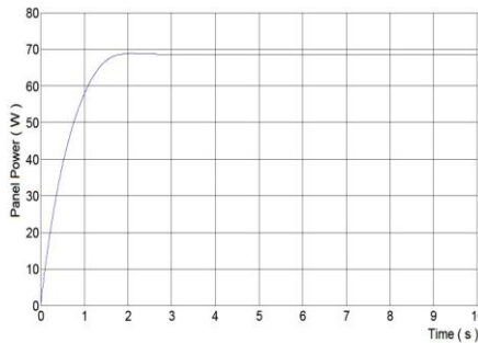
Fig. 5-a: Simulation results of the systems under constant conditions (standard) A temperature of 25 °C and an irradiation of 1000 W/m 2
