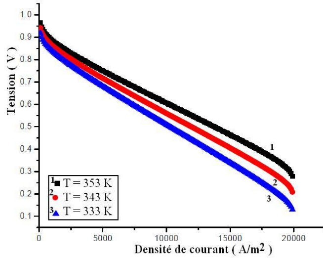
Fig. 2: Polarization curve at different values of temperature
