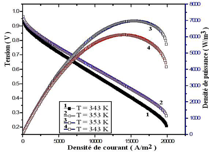
Fig. 5: Effect of temperature on the polarization curve of the PEM fuel cell
