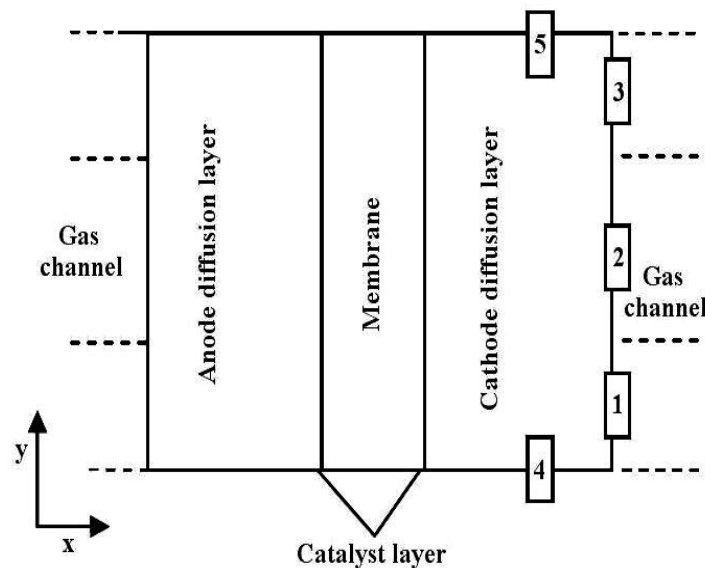
Fig. 1: Schematic diagram of PEM fuel cell modeling regions
