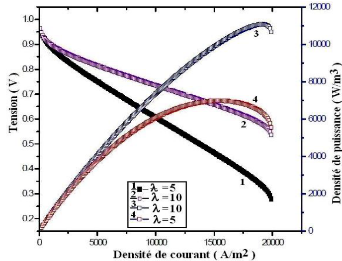
Fig. 6: Effect of water content on the polarization curve of the PEM fuel cell
