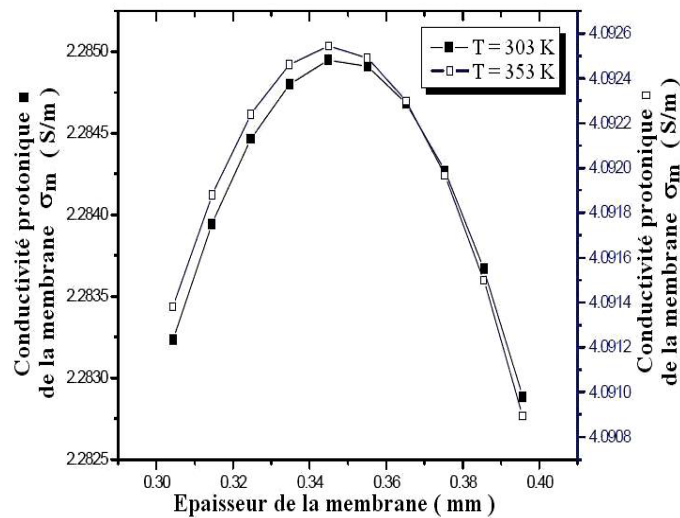
Fig. 3: Proton conductivity of the membrane for different values of temperature
