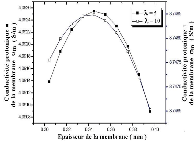
Fig. 4: Proton conductivity of the membrane in different values of the water content
