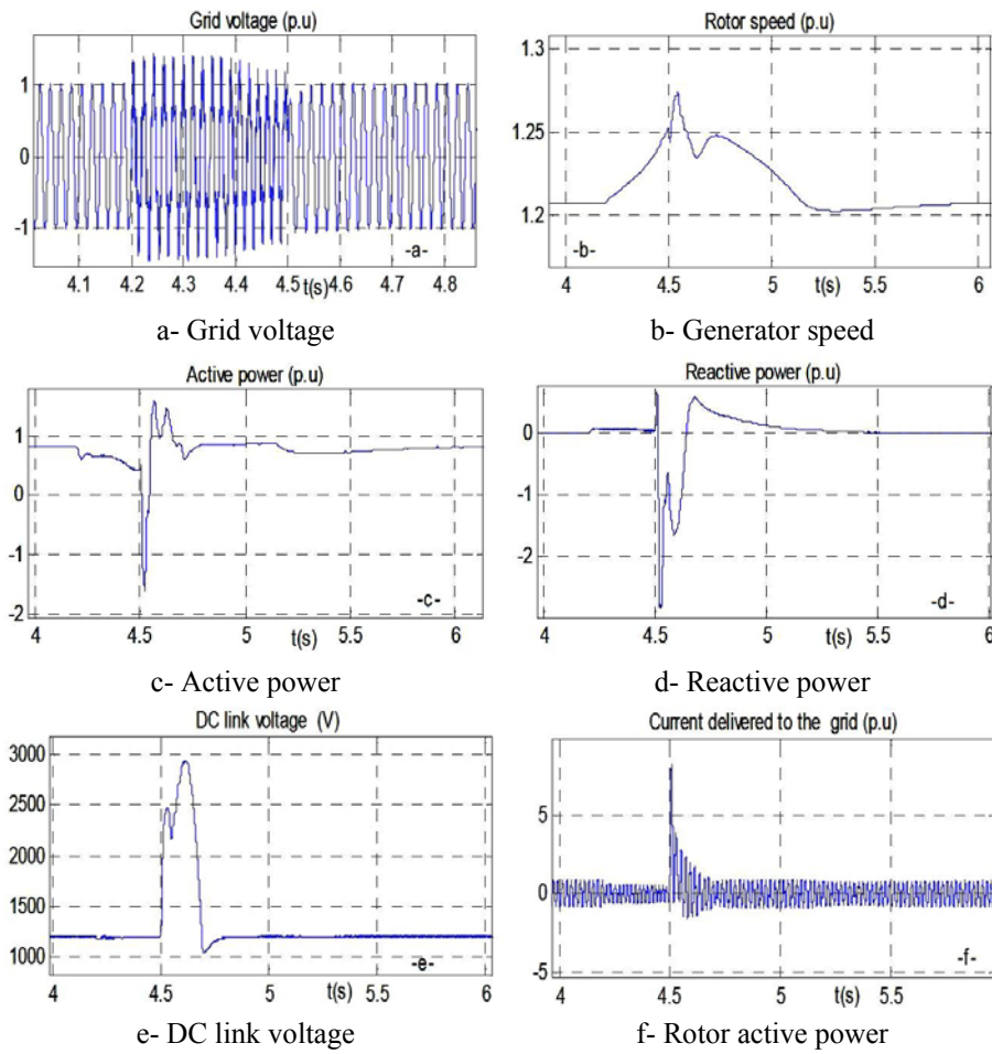
Fig. 12: Results obtained with a PI regulator
