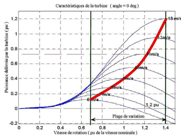
Fig. 3: Turbine characteristics
