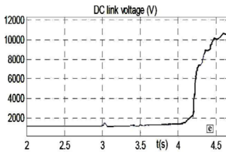
e- DC link voltage
