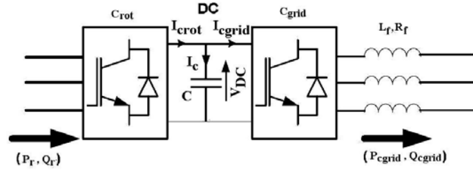
Fig. 4: Unified Power Flow Controllers, 'UPFC'
