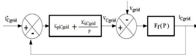
Fig. 7: C_{grid} Converter current regulation block diagram
