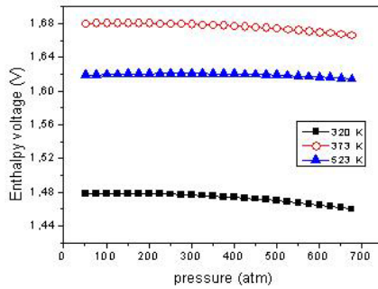
Fig. 5: Enthalpy voltage against pressure and temperature variations
