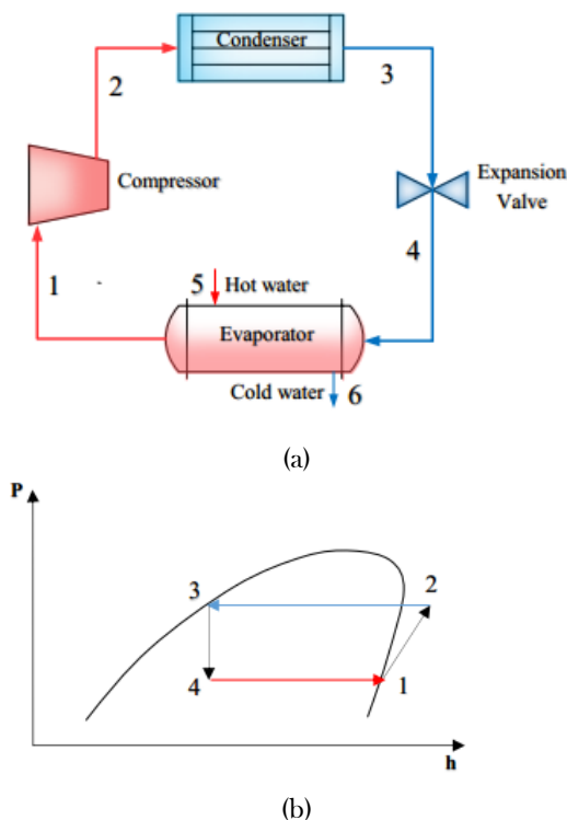
Figure 1. Schematic diagram (a) and P-h diagram (b) of the conventional refrigeration cycle [13]
