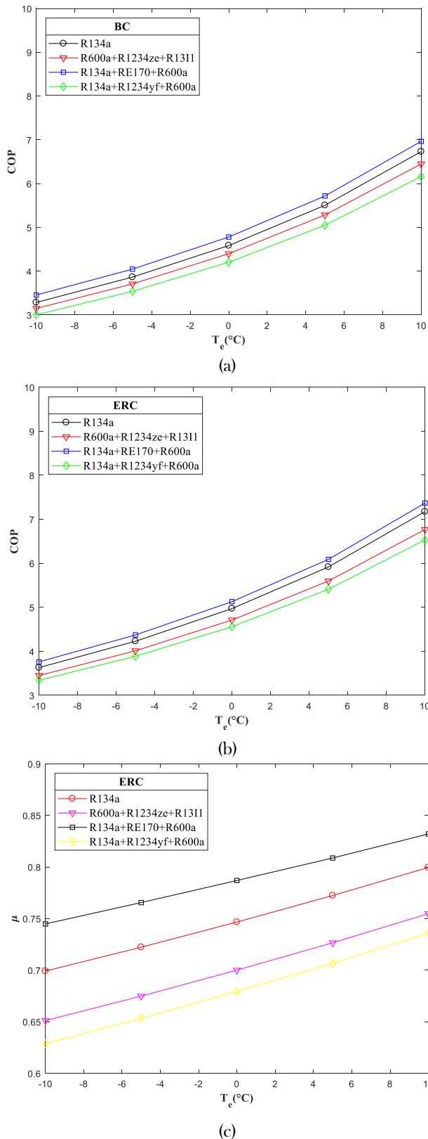
Figure 5. Influence of the variation of the evaporation temperature on the performance of the cycles
