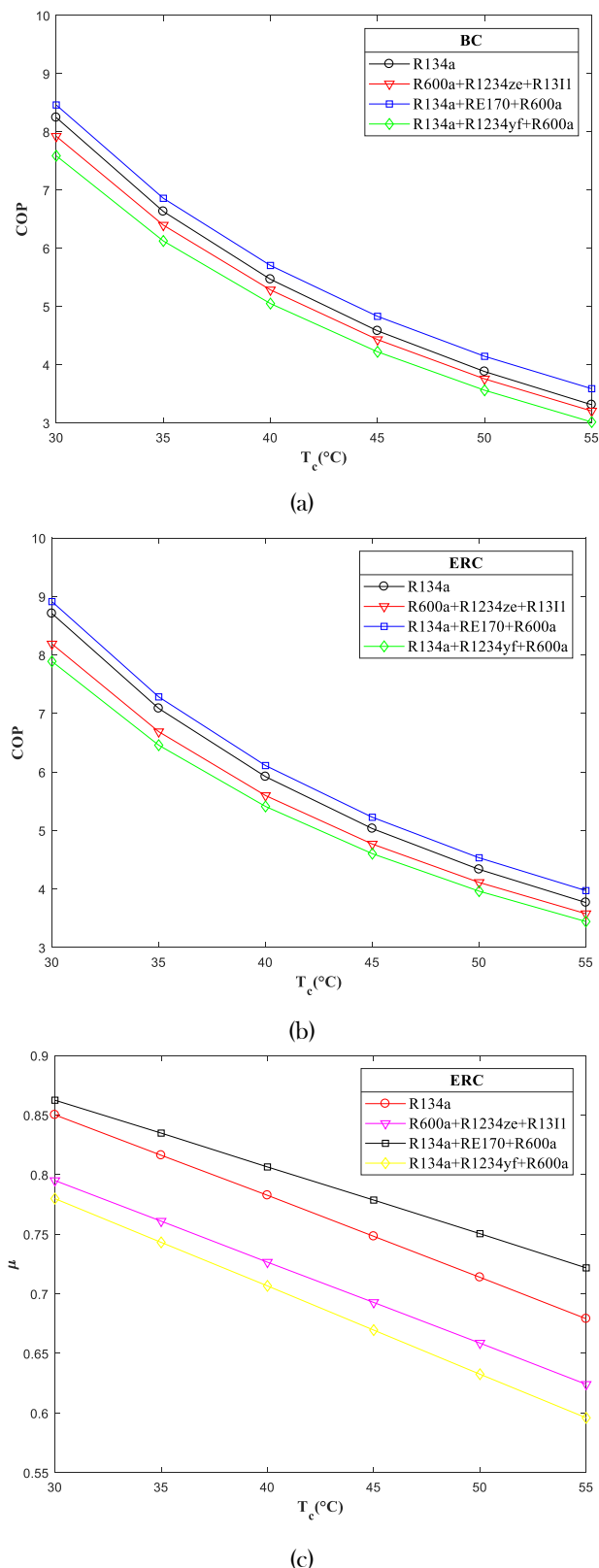
Figure 4. Influence of the variation of the condensing temperature on the performance of the cycles
