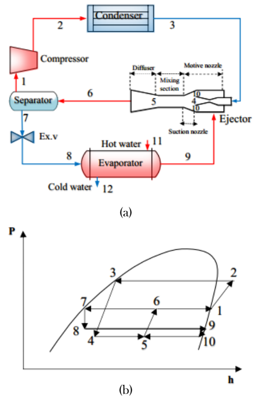
Figure 2. Schematic diagram (a) and P-h diagram (b) of the compression / ejector refrigeration cycle [7]
