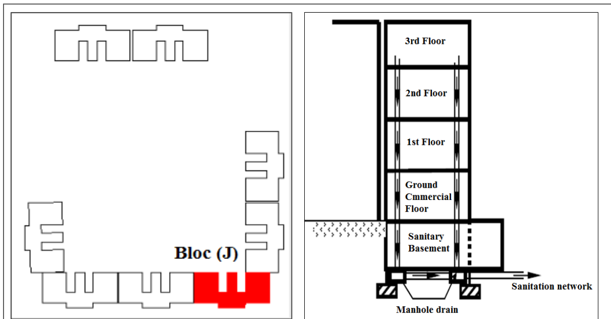
Fig 2. Situation and general structure of Bloc (J) building.
