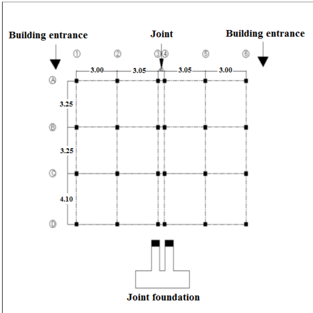
Fig 4. Foundation plan of the building.
