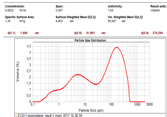
Figure 3. Granulometric distribution of porcelain powder
