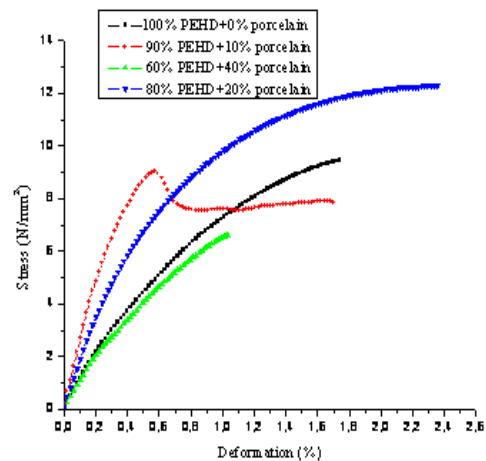
Figure 6. Stress deformation curve for HDPE samples with (0, 10, 20, 40wt. % of porcelain)
