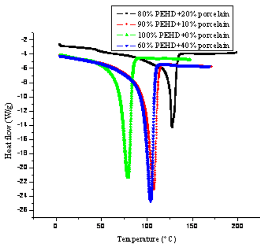
Figure 5. DSC thermograms obtained on composite HDPE-porcelain
