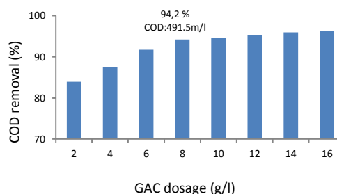
Figure 8. Activated carbon adsorption as post treatment after coagulation and Fenton oxidation
