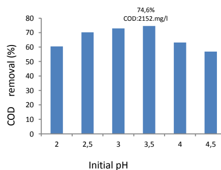
Figure 6. Effect of initial pH on COD removal efficiency (Conditions: H_2O_2 =5g/l, H_2O_2 /Fe (II) molar ratio=6; original COD =8474.7mg/l)
