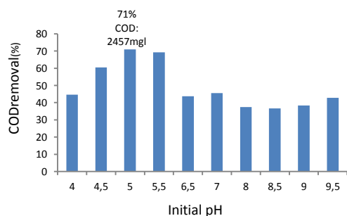
Figure 3. Effect of initial pH on COD removal efficiency ( \text{FeCl}_3=1.6\text{g/l} ; original COD 8474.72 mg/l)
