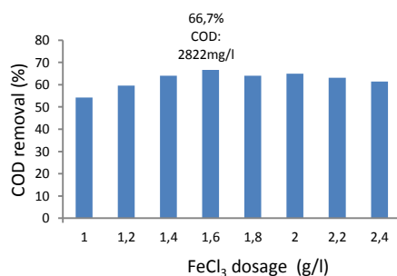
Figure 2. Effect of coagulant dosing on COD removal efficiency (pH=4.5; original COD =8474.7 mg/l)
