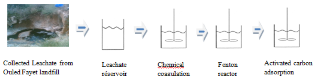
Figure1. Flow process of the three treatment units of landfill leachate (coagulation, Fenton and activated carbon adsorption)
