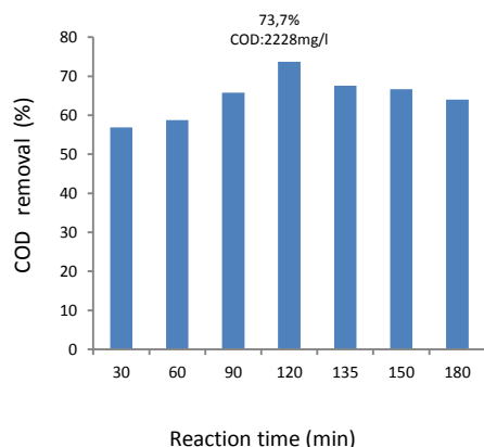
Figure 7. Effect of reaction time on COD removal efficiency (conditions: initial pH= 3.5; H_2O_2 = 5g/l; H_2O_2/Fe (II) molar ratio=6, original COD=8474.7 mg/l)
