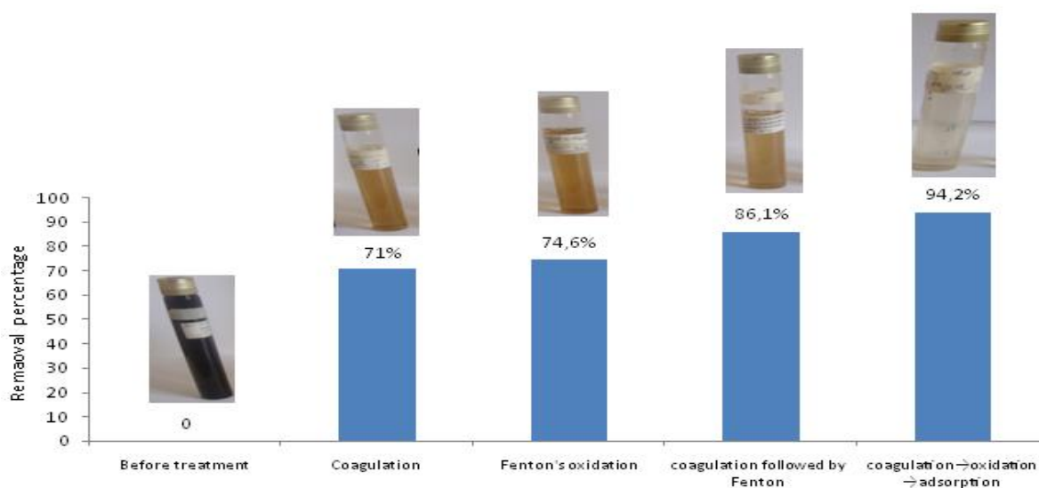
Figure 9. Chemical oxygen demand (COD) removal efficiencies against treatment stages
