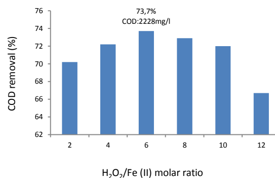
Figure 4. Effect of \text{H}_2\text{O}_2 / Fe (II) molar ratio on COD removal efficiency (conditions: initial pH= 3; \text{H}_2\text{O}_2= 5\text{g/l} ; original COD=8474.7 mg/l)
