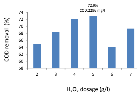
Figure 5. Effect of H_2O_2 dosing on COD removal efficiency (conditions: Initial pH 3; H_2O_2 /Fe (II) molar ratio=6; original COD 8474.7 mg/l)
