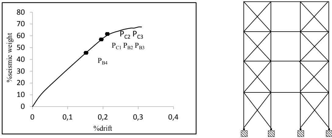
Fig.5 - Pushover curve for RC bracing in alternate bay
