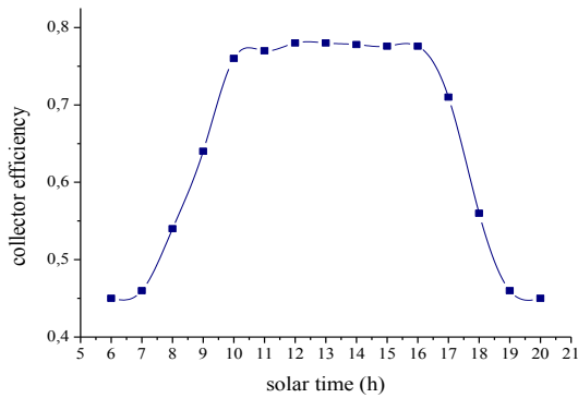
Fig. 8, Variations of collector efficiency during design day for July
