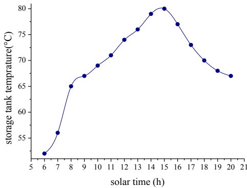
Fig. 5, Temperature distribution of storage tank for design day of July
