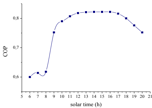
Fig. 9, Variations of COP during design days for July
